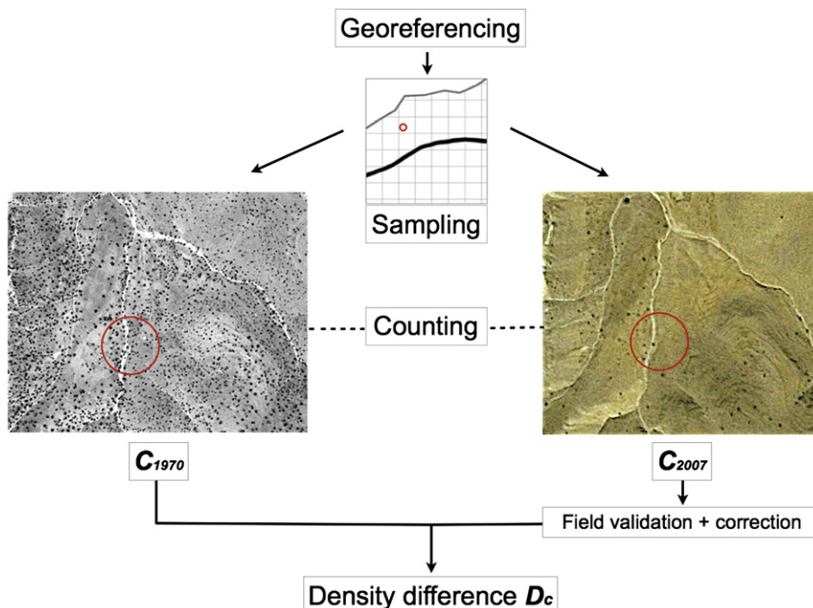
Fig. 3. Counting Method.
